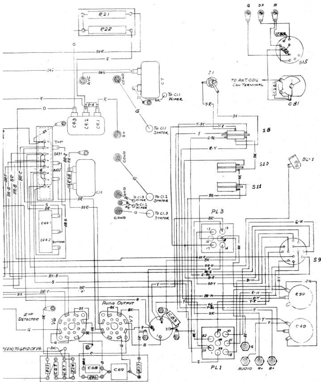
TYPE RA-IB RECEIVER WIRING DIAGRAM
