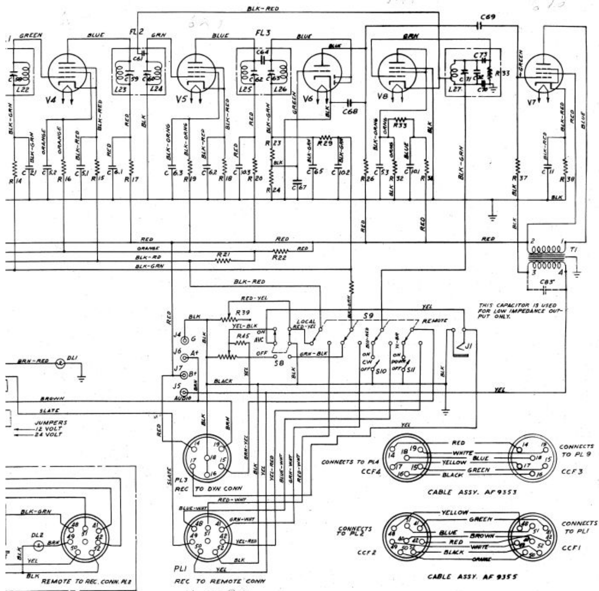
FIG.15- TYPE RA-1B RECEIVER UNIT SCHEMATIC DIAGRAM
