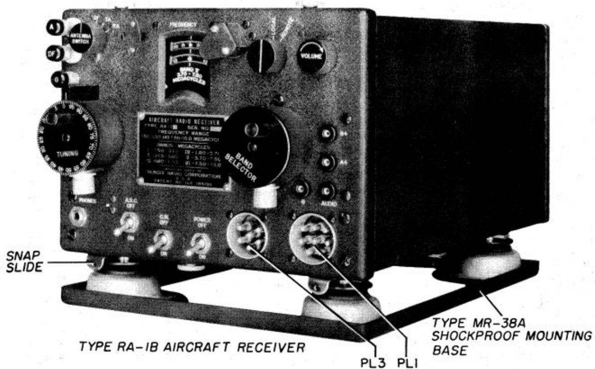
FIG. 1—TYPE RA-1B AIRCRAFT RADIO RECEIVER EQUIPMENT
